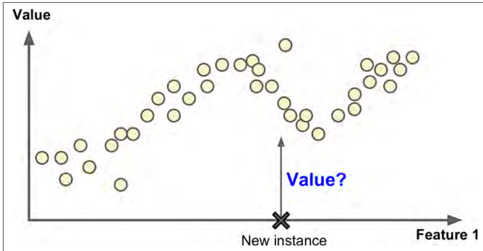
Figure 1-6. Regression
