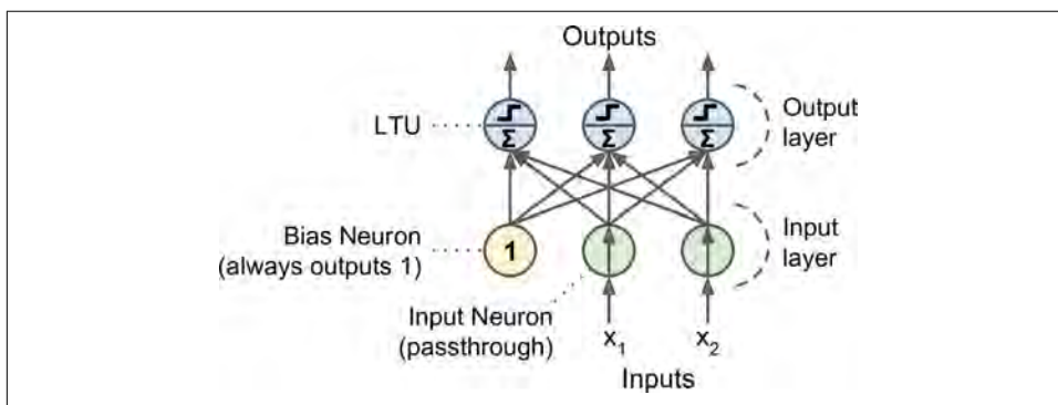
Figure 10-5. Perceptron diagram
